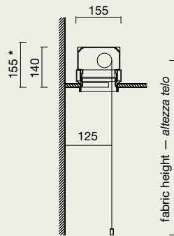
Fabric lowering: front (standard) Discesa telo: avanti (standard)
