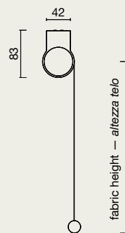
Fabric lowering: front (standard) Discesa telo: avanti (standard)
