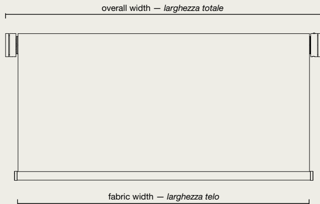
Front view Vista frontale
