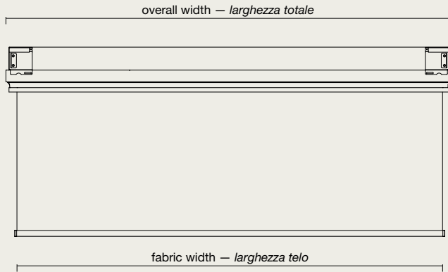
Front view Vista frontale
